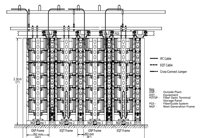
Cross-connect application using 8-inch wide FOTSP in a 1:1 application (1 Equipment to 1 OSP)
