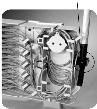
72-position FTB loaded with multifiber breakout cable
