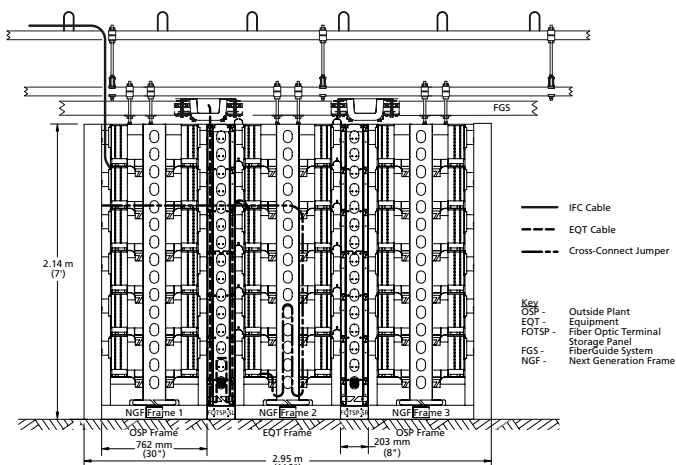
Cross-connect application using 8-inch wide FOTSP in a 2:1 application (2 Equipment to 1 OSP)
