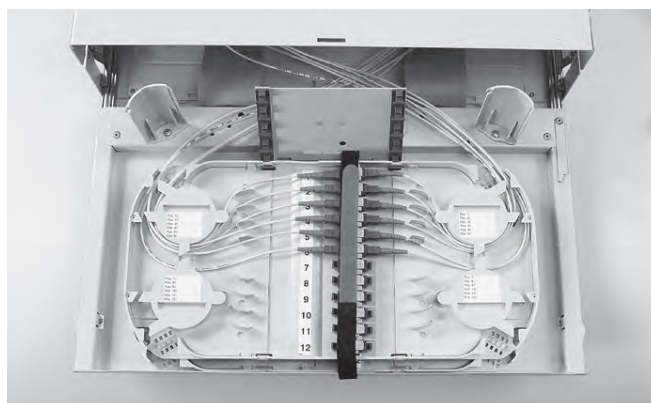
7.3 Routing of incoming pigtails and outgoing patchcords.
